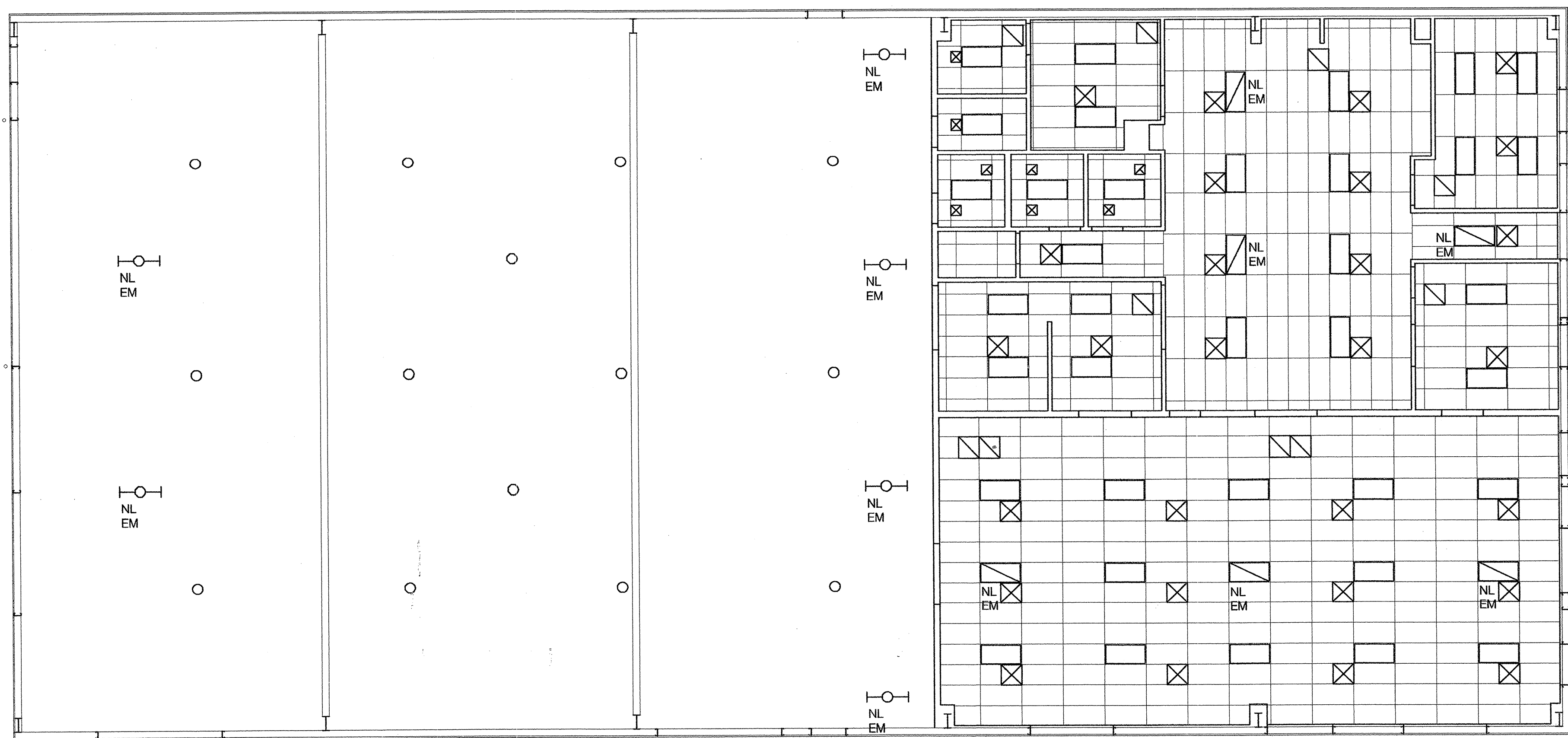
Reflected Ceiling Plan North 1/8" = 1'-0"
