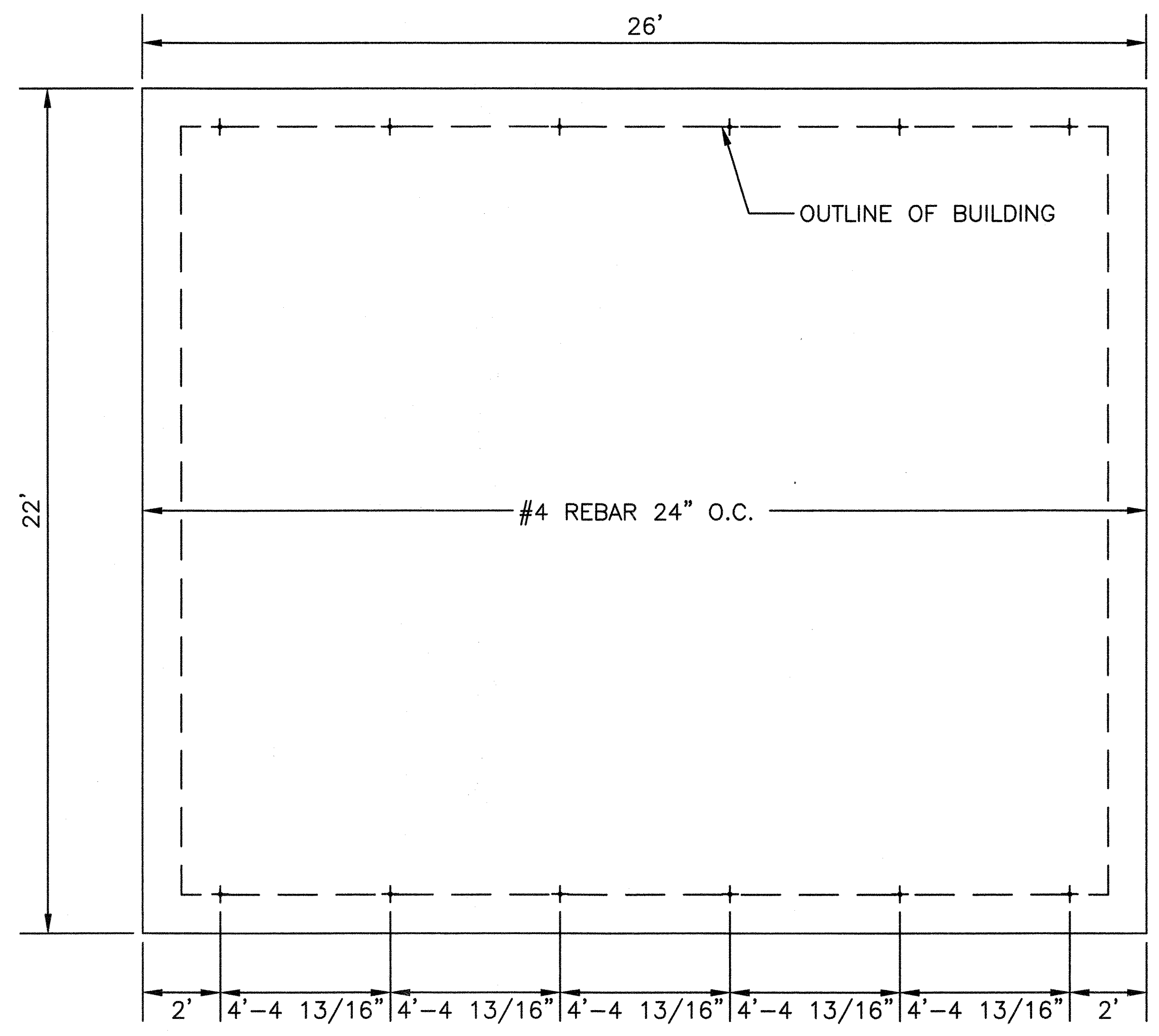
PLAN VIEW
